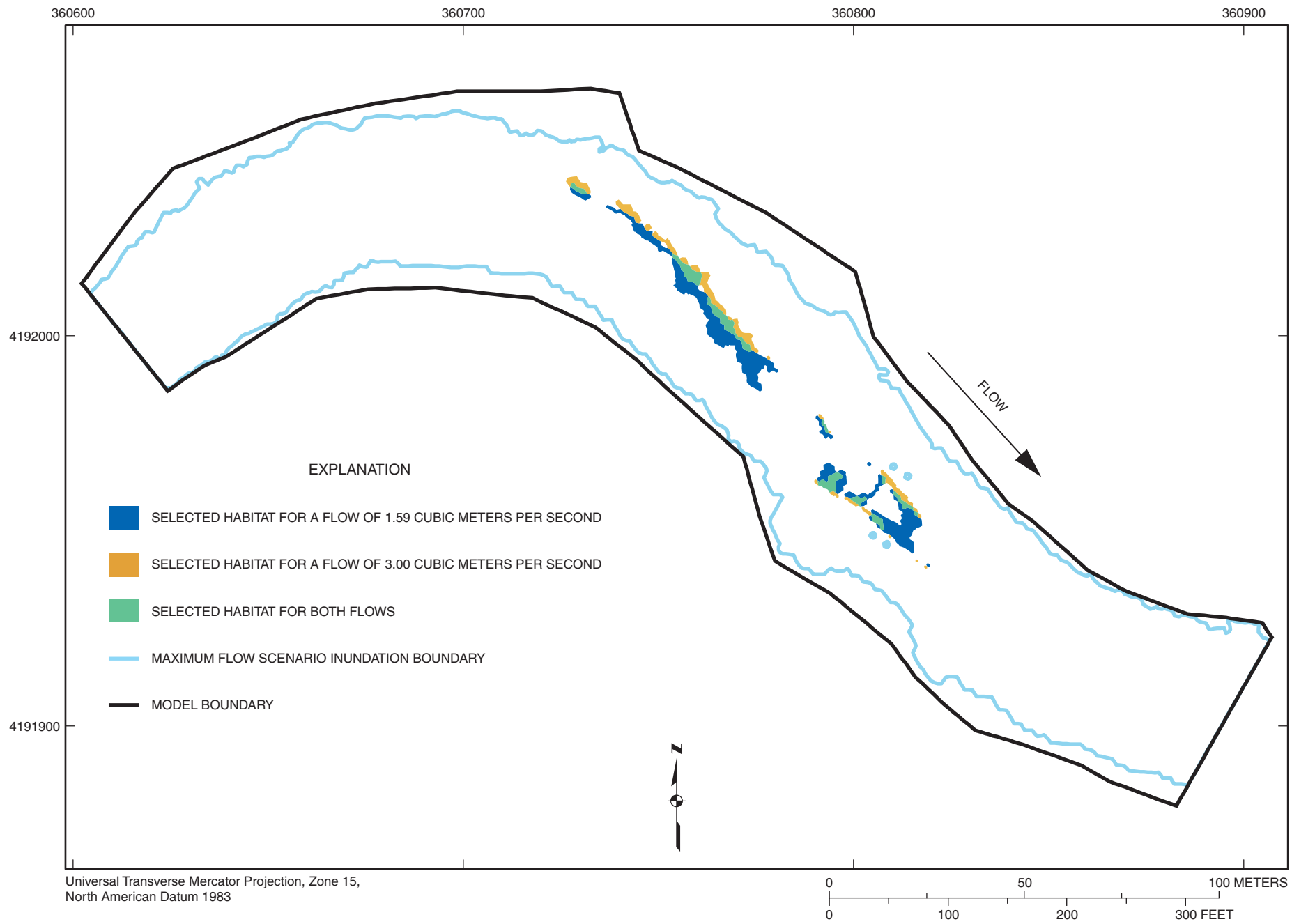
Figure 1-33. Selected habitat area distribution for habitat category 14 (flathead catfish) at flows of 1.59 and 3.00 cubic meters per second at Marmaton River site M1.
